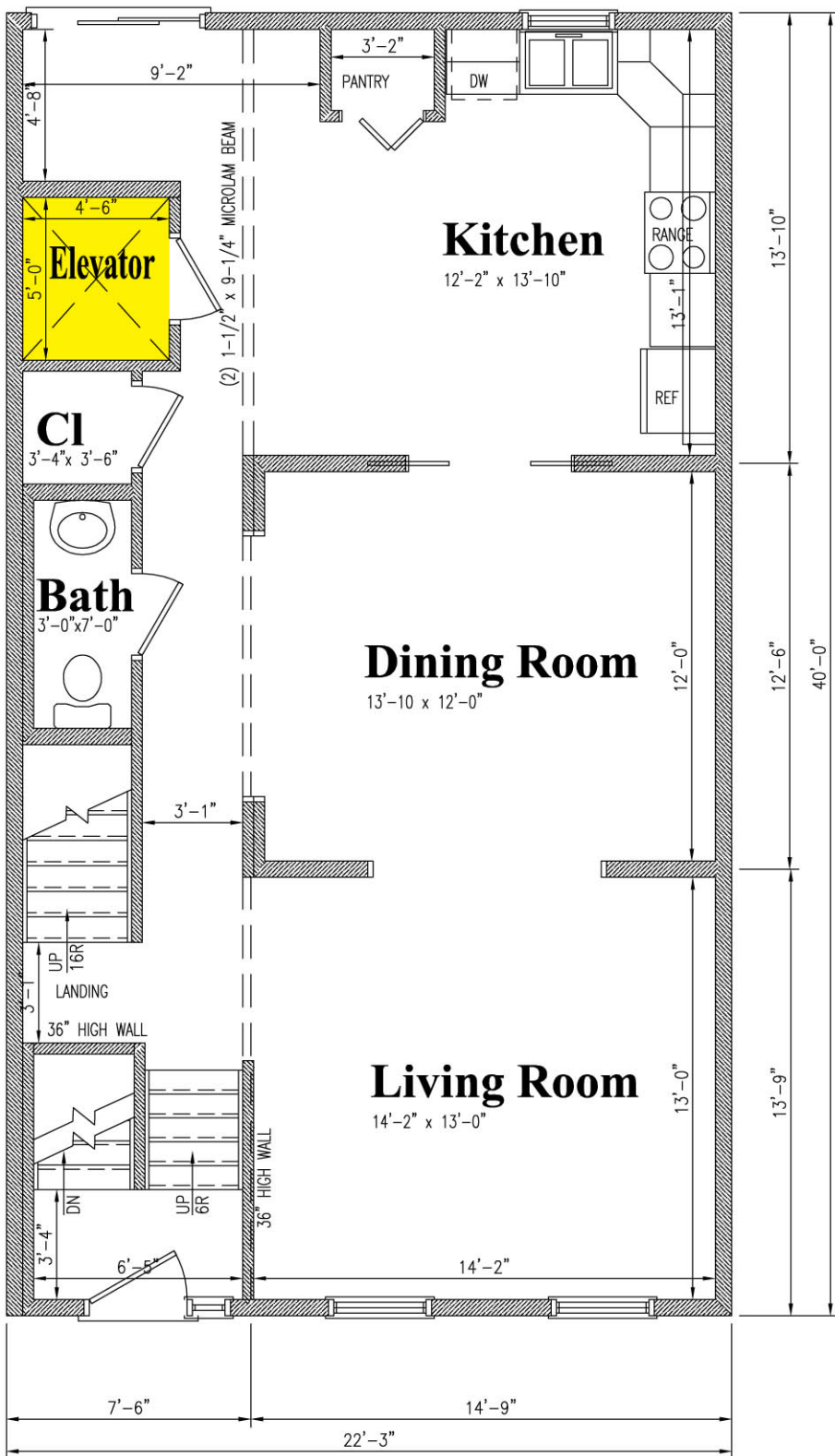
2 First Floor Plan - 897 sf A2 Scale: 1/4"=1'-0"
