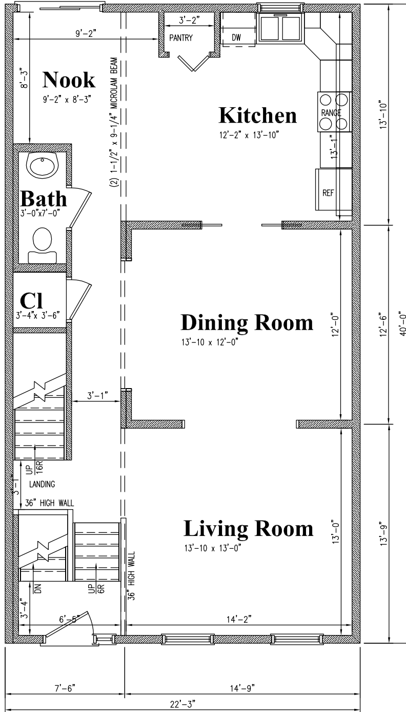
2 First Floor Plan - 897 sf A2 Scale: 1/4"=1'-0"
